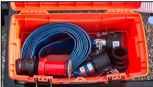
The toolbox comes loaded with 25' of lay flat hose with quick coupler fittings, a fire hydrant adapter, and an adjustable water nozzle
